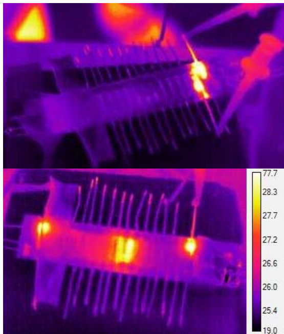
Figure 7: Thermographic images of impacted FFRP specimen. (Top) shows electrodes away from damage without any anomalies. (Bottom) Large anomaly is visible when electrode pair spans impact-damaged region. (Scale in degrees Celsius)
